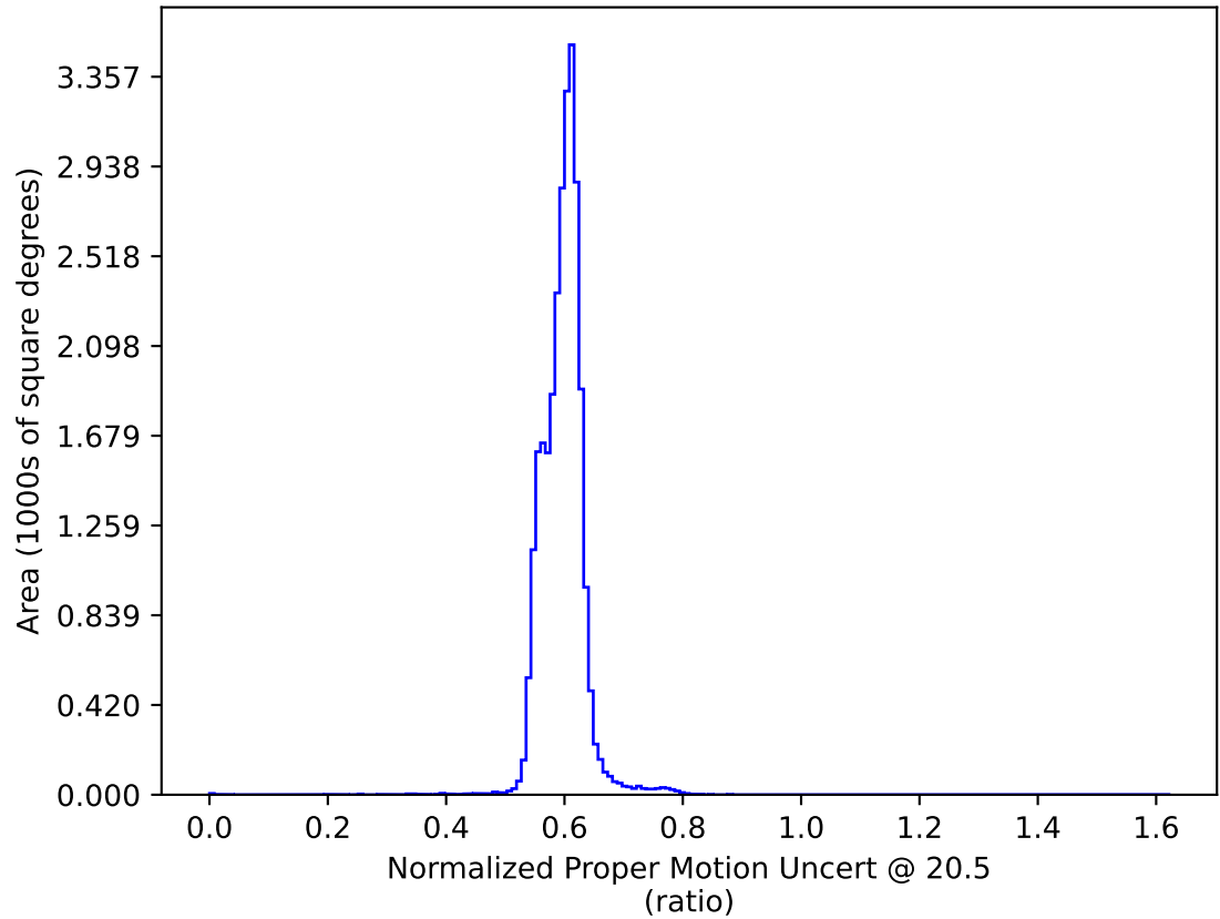
ddf_acor_sf10_lsf40_lsr20_v3.4_10yrs All sky: Normalized Proper Motion Uncert @ 20.5
