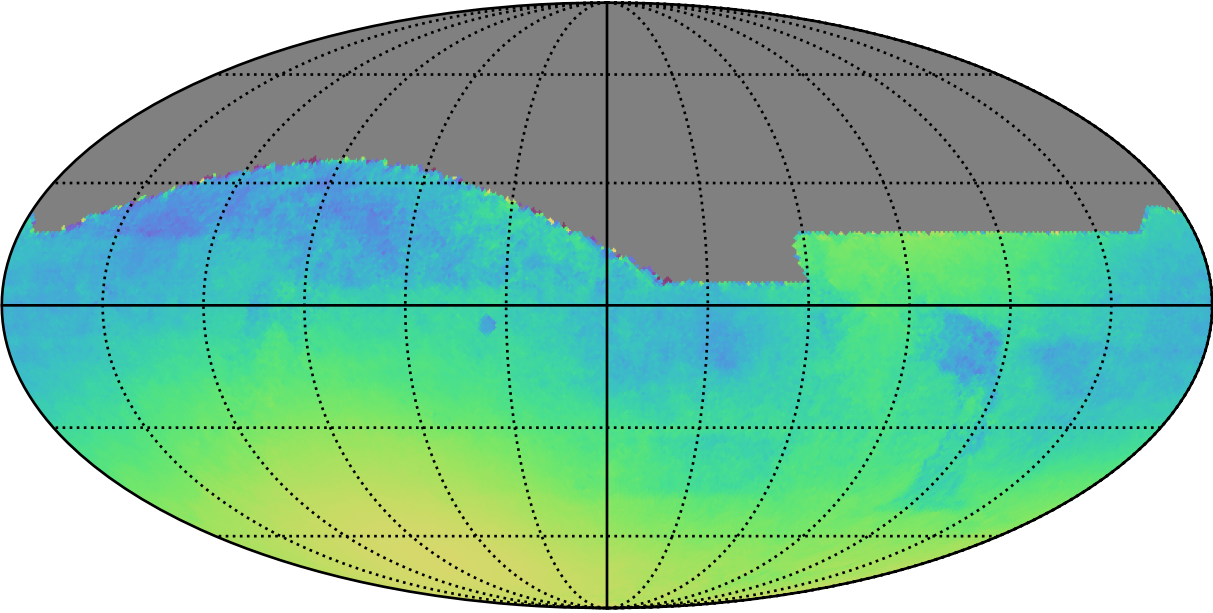
ddf_acor_sf10_lsf40_lsr20_v3.4_10yrs All sky: Normalized Parallax Uncert @ 24.0
