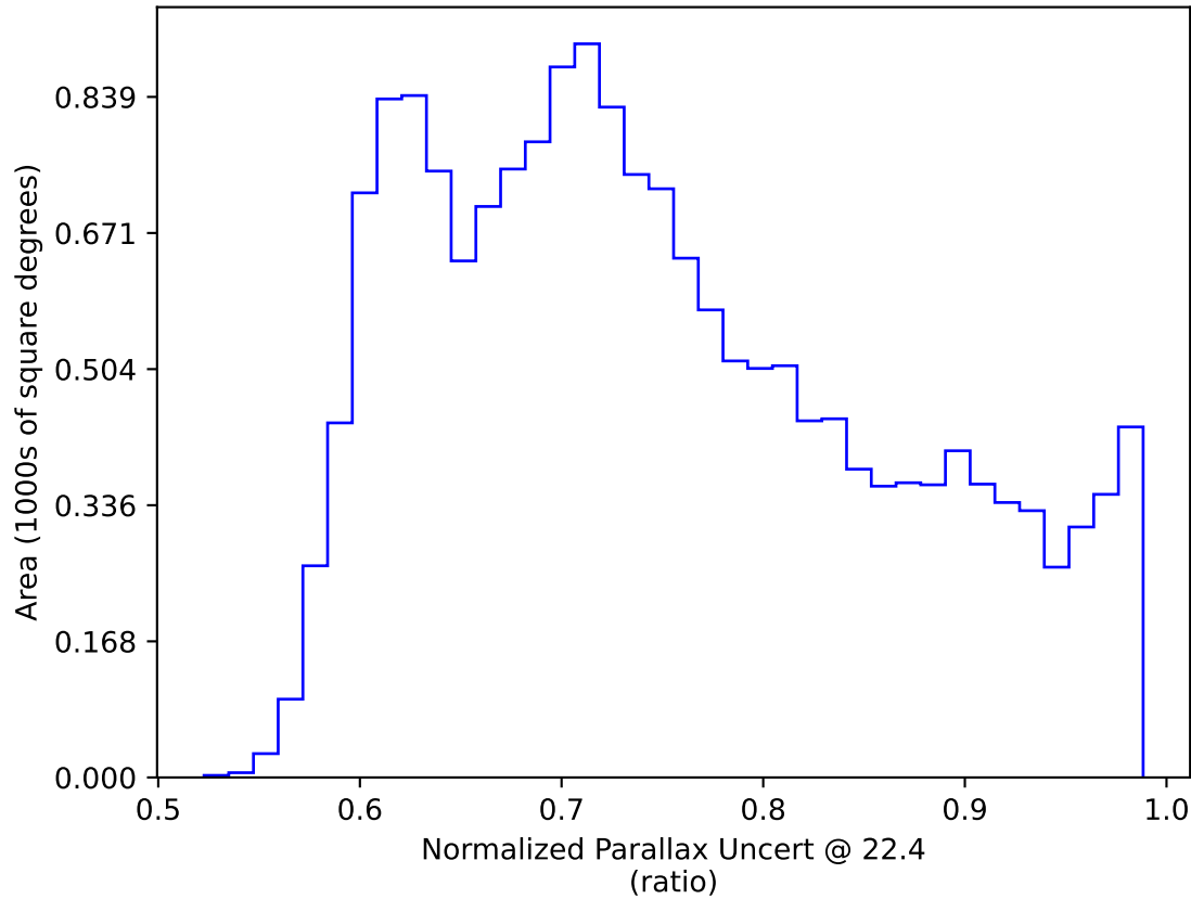
ddf_acor_sf10_lsf40_lsr20_v3.4_10yrs WFD: Normalized Parallax Uncert @ 22.4
