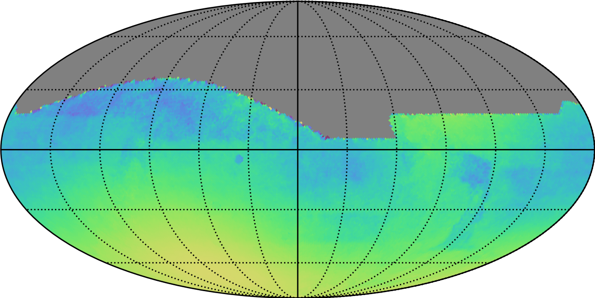
ddf_acor_sf10_lsf40_lsr20_v3.4_10yrs All sky: Normalized Parallax Uncert @ 22.4
