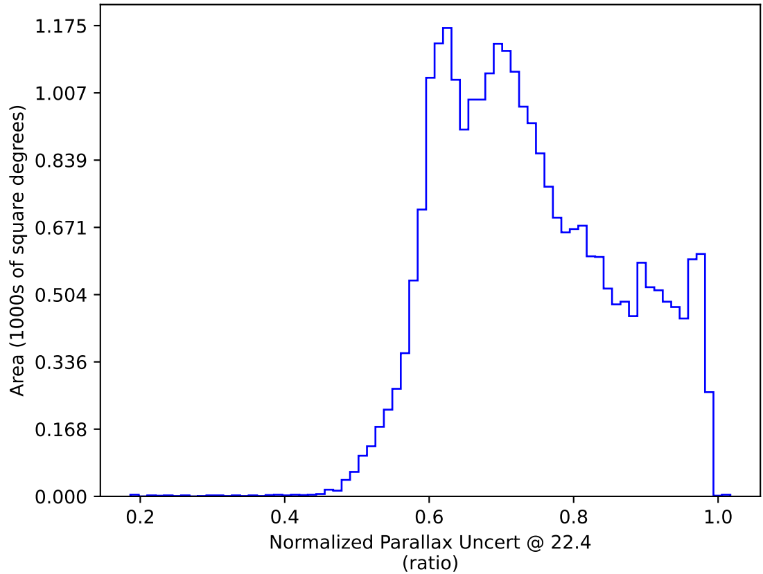
ddf_acor_sf10_lsf40_lsr20_v3.4_10yrs All sky: Normalized Parallax Uncert @ 22.4
