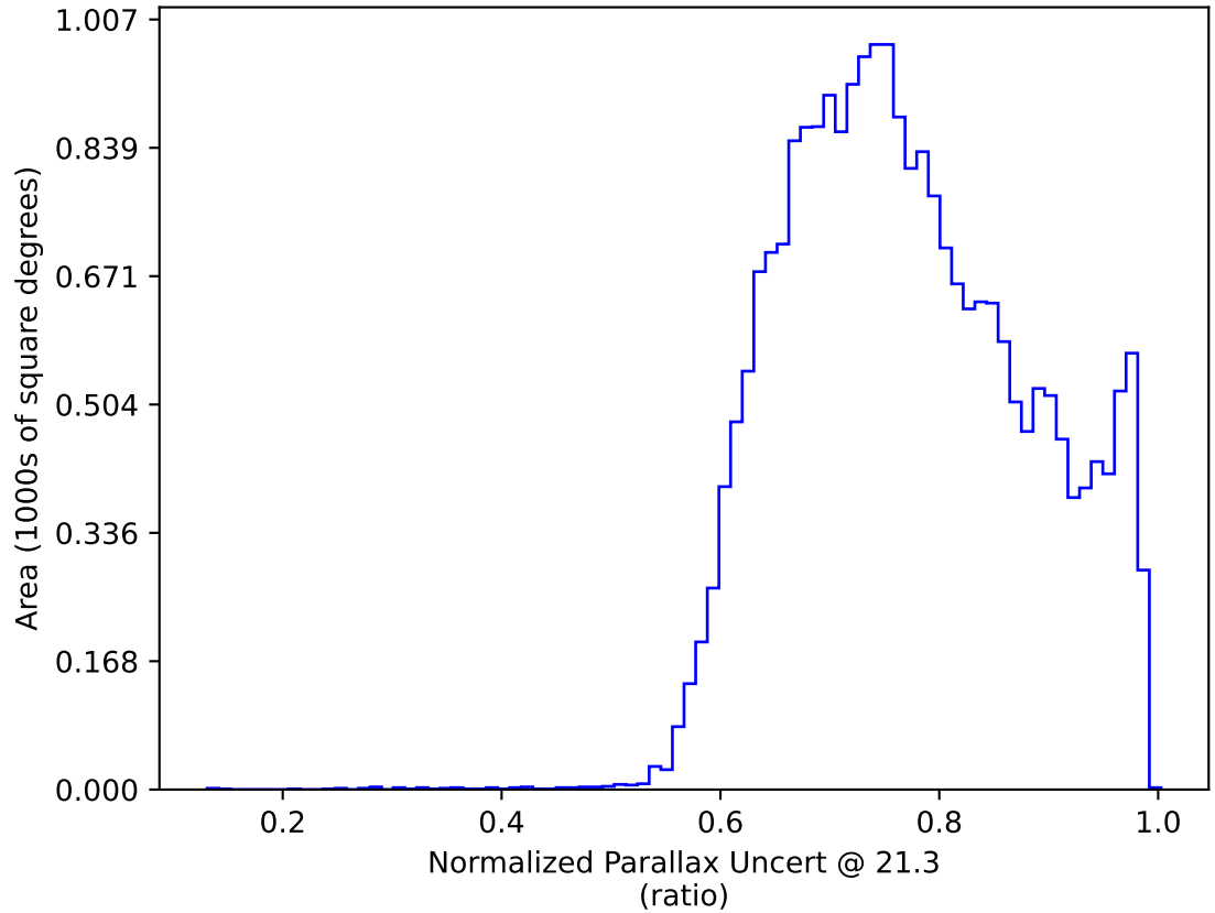
ddf_acor_sf10_lsf40_lsr20_v3.4_10yrs All sky y band only: Normalized Parallax Uncert @ 21.3
