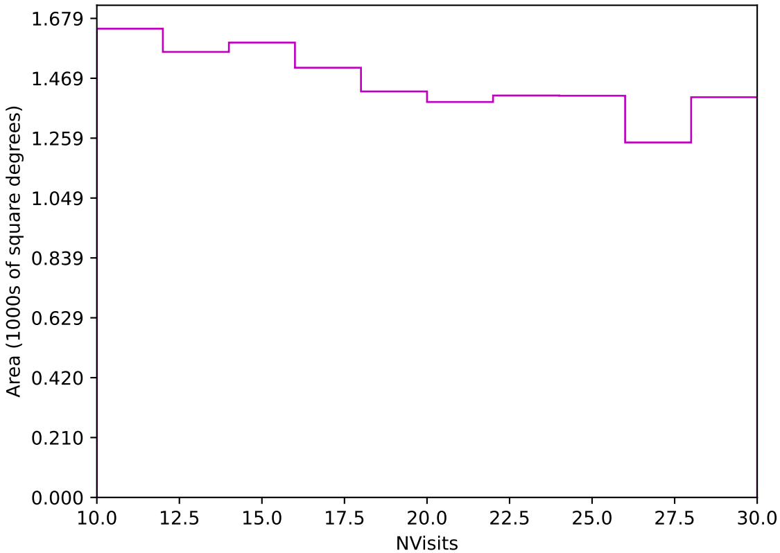
ddf_acor_sf10_lsf40_lsr20_v3.4_10yrs Yr 3-4 z band: NVisits
