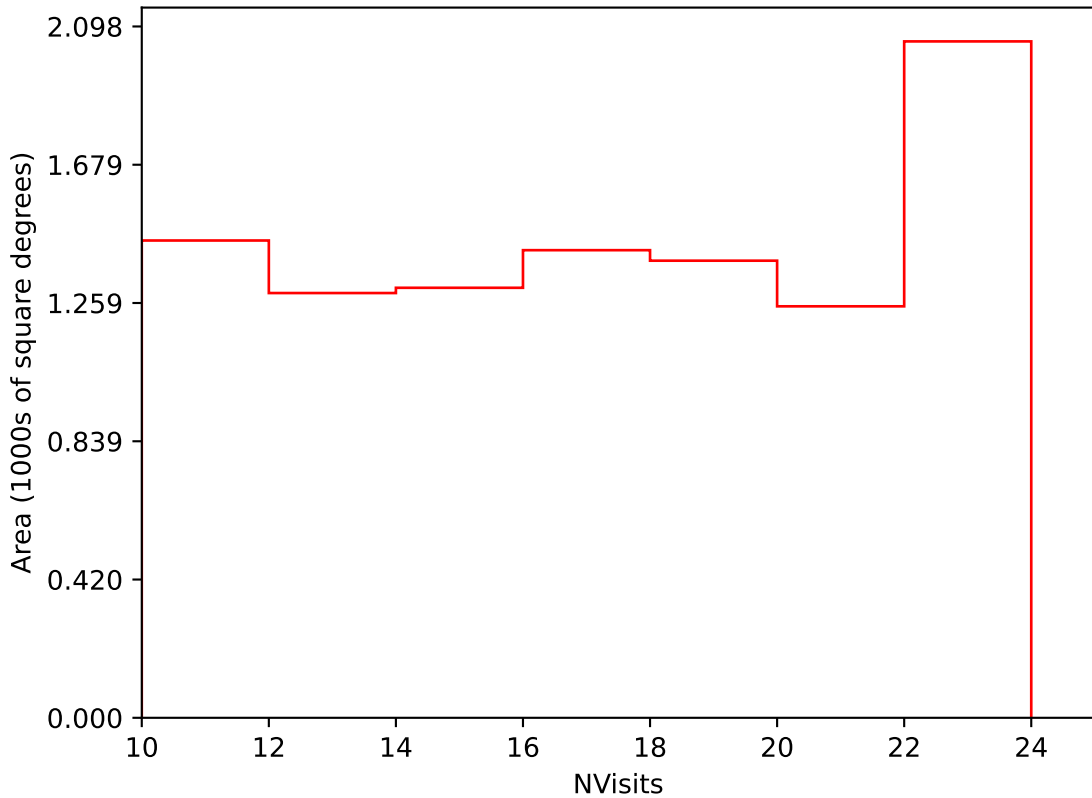
ddf_acor_sf10_lsf40_lsr20_v3.4_10yrs Yr 3-4 i band: NVisits
