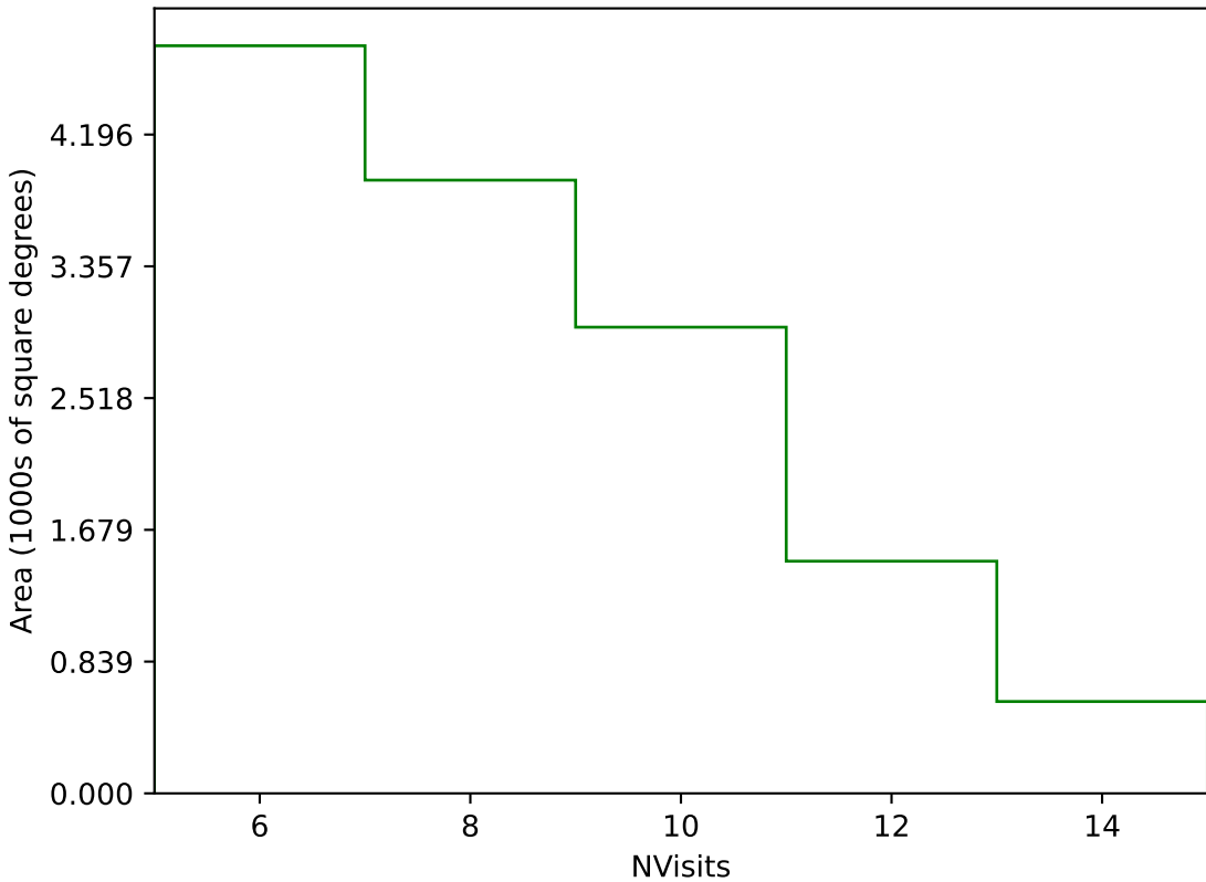
ddf_acor_sf10_lsf40_lsr20_v3.4_10yrs Yr 3-4 g band: NVisits
