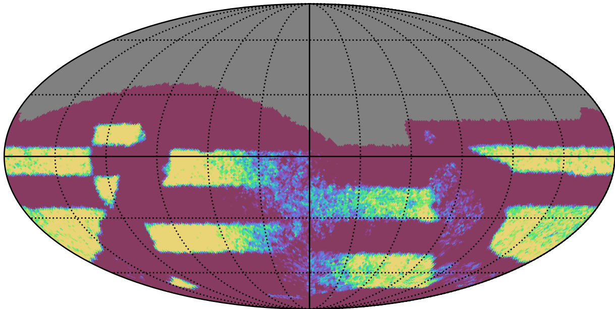
ddf_acor_sf10_lsf40_lsr20_v3.4_10yrs Yr 3-4 all bands: NVisits
