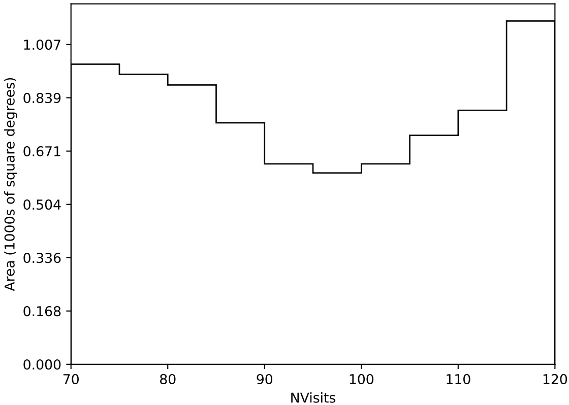
ddf_acor_sf10_lsf40_lsr20_v3.4_10yrs Yr 3-4 all bands: NVisits
