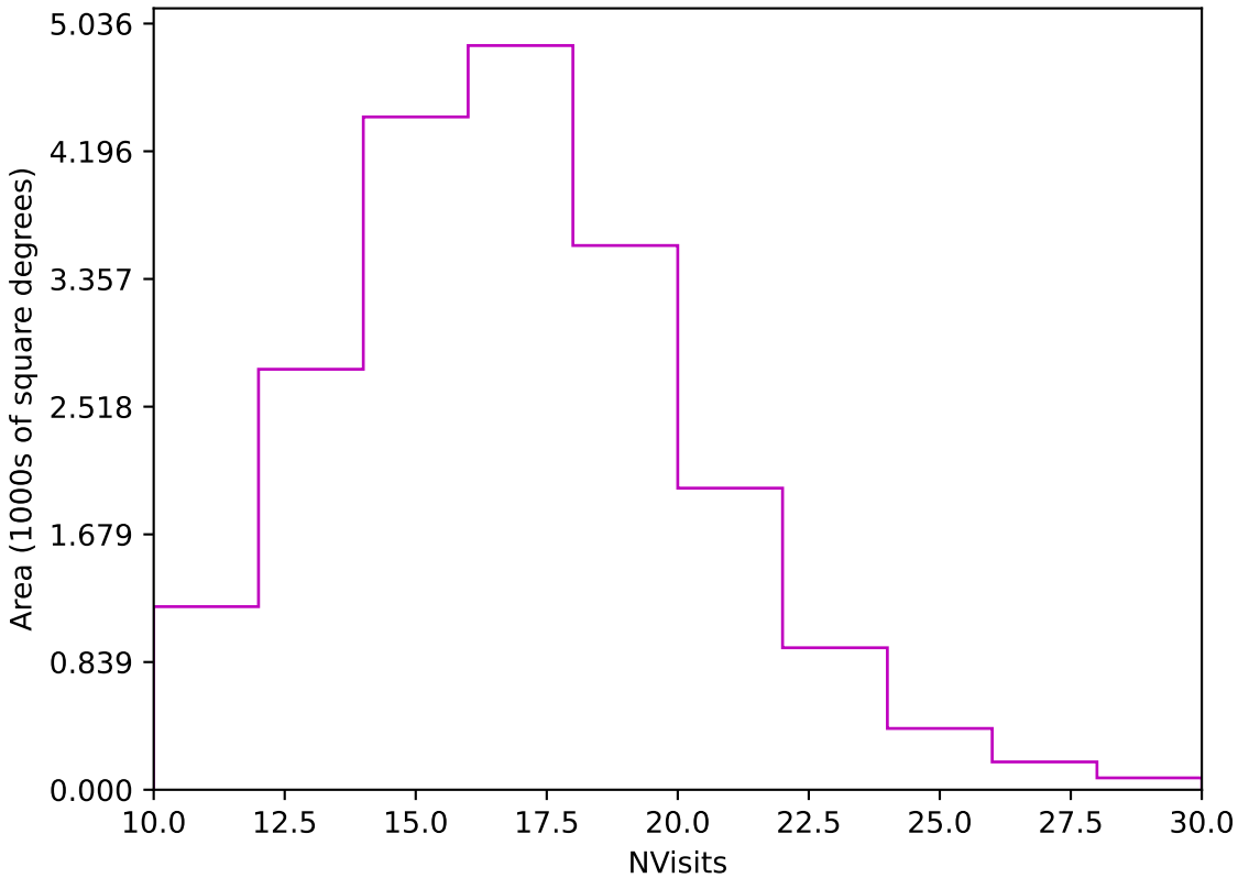
ddf_acor_sf10_lsf40_lsr20_v3.4_10yrs Yr 1 z band: NVisits
