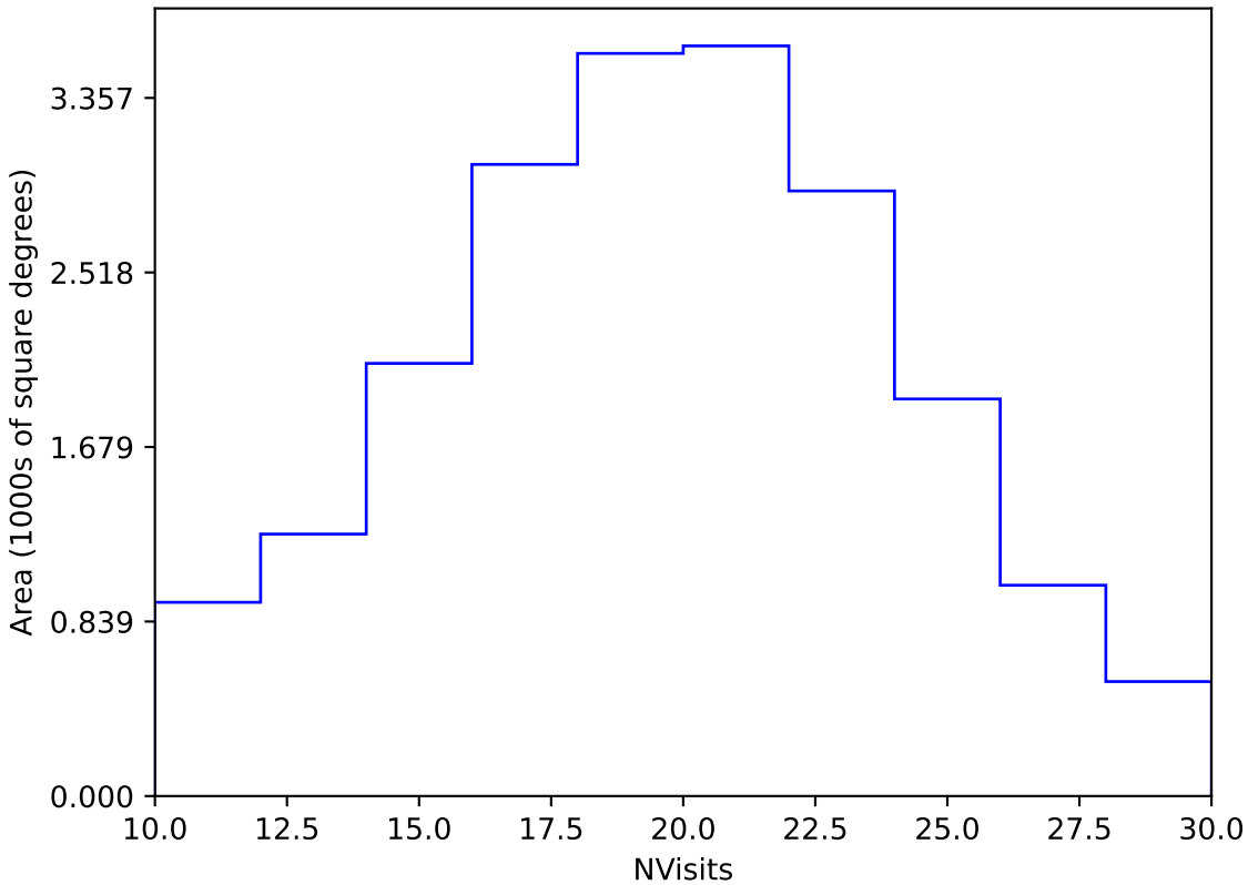
ddf_acor_sf10_lsf40_lsr20_v3.4_10yrs Yr 1 y band: NVisits
