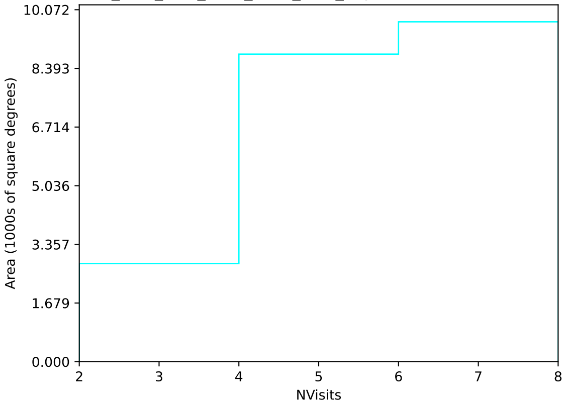
ddf_acor_sf10_lsf40_lsr20_v3.4_10yrs Yr 1 u band: NVisits
