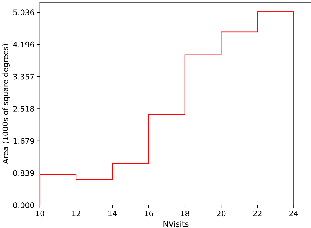
ddf_acor_sf10_lsf40_lsr20_v3.4_10yrs Yr 1 i band: NVisits
