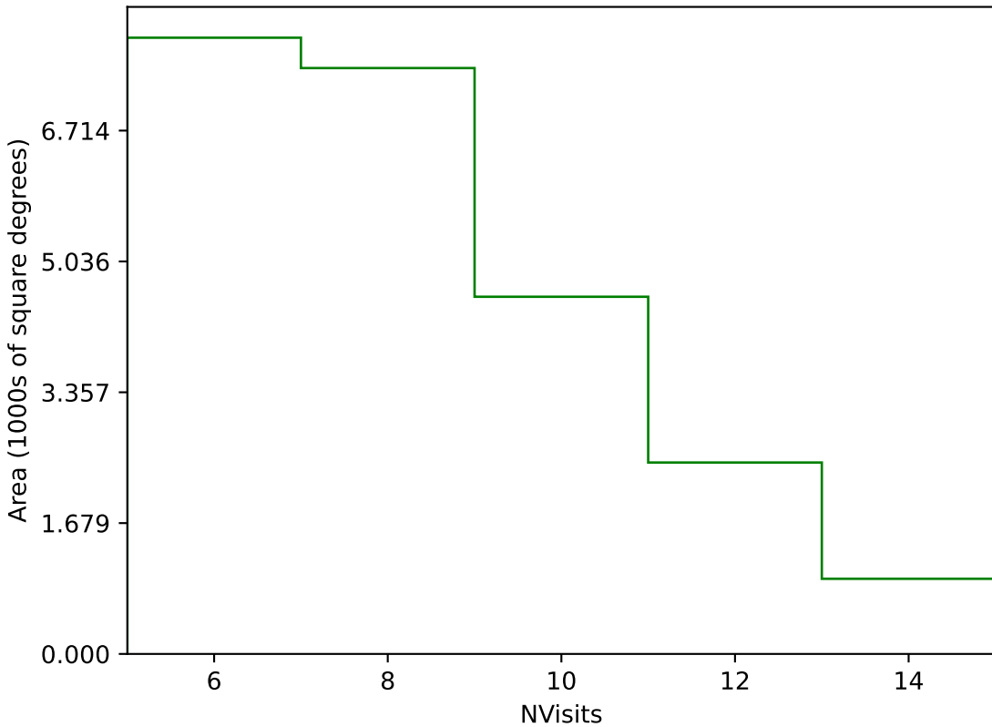
ddf_acor_sf10_lsf40_lsr20_v3.4_10yrs Yr 1 g band: NVisits
