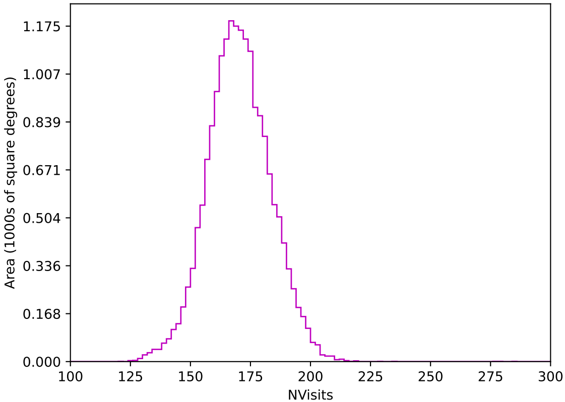
ddf_acor_sf10_lsf40_lsr20_v3.4_10yrs WFD z band: NVisits
