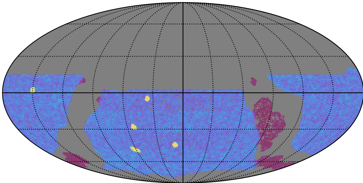
ddf_acor_sf10_lsf40_lsr20_v3.4_10yrs WFD y band: NVisits
