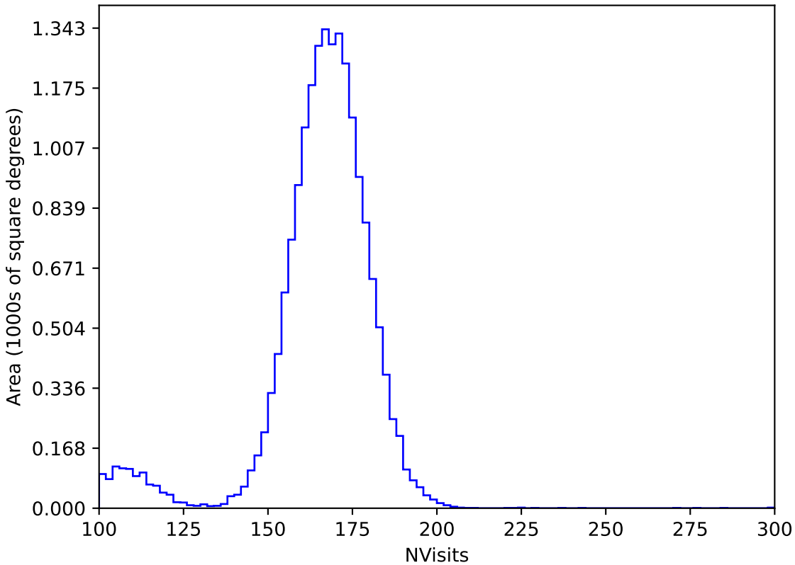
ddf_acor_sf10_lsf40_lsr20_v3.4_10yrs WFD y band: NVisits
