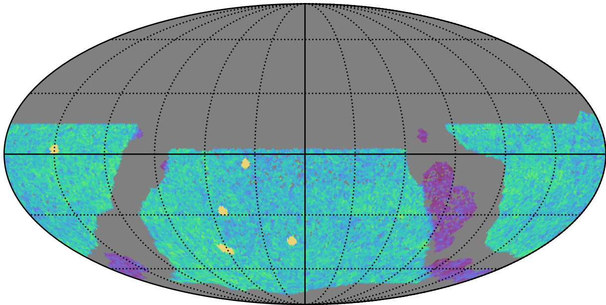
ddf_acor_sf10_lsf40_lsr20_v3.4_10yrs WFD u band: NVisits
