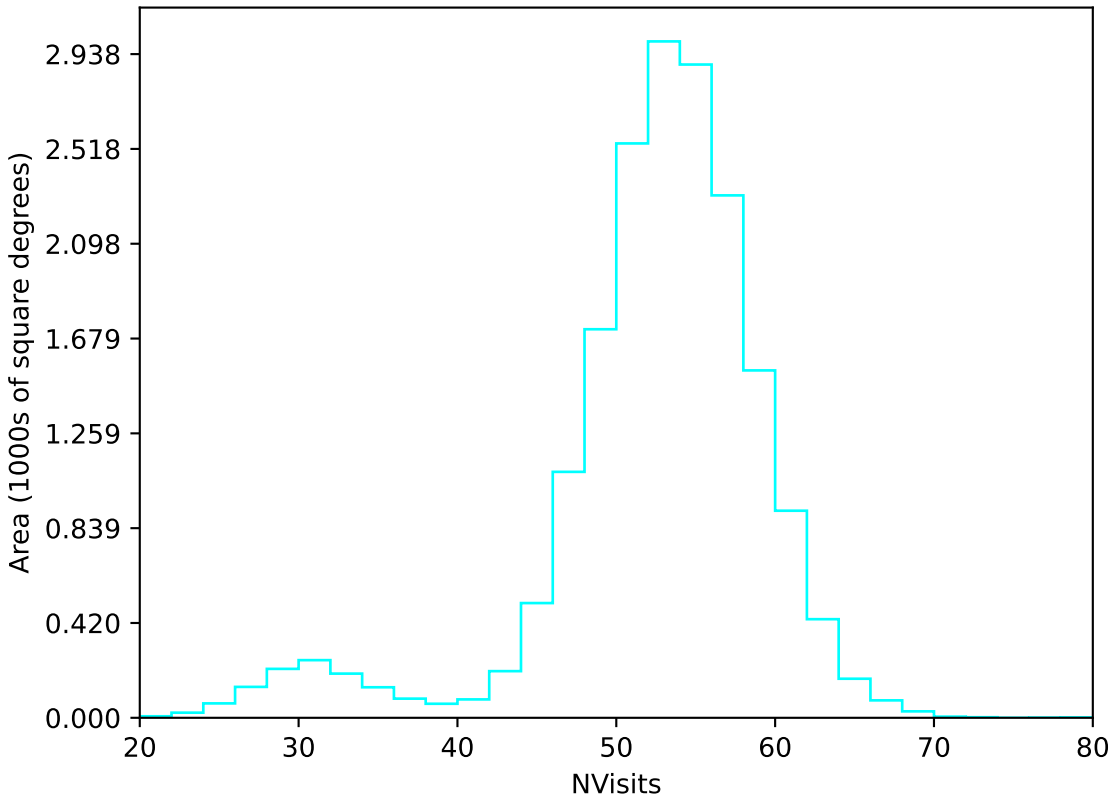
ddf_acor_sf10_lsf40_lsr20_v3.4_10yrs WFD u band: NVisits
