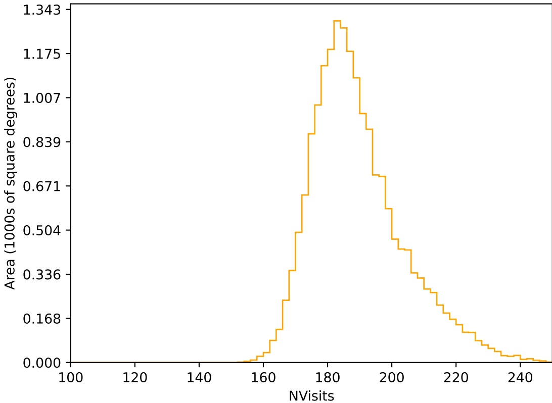
ddf_acor_sf10_lsf40_lsr20_v3.4_10yrs WFD r band: NVisits
