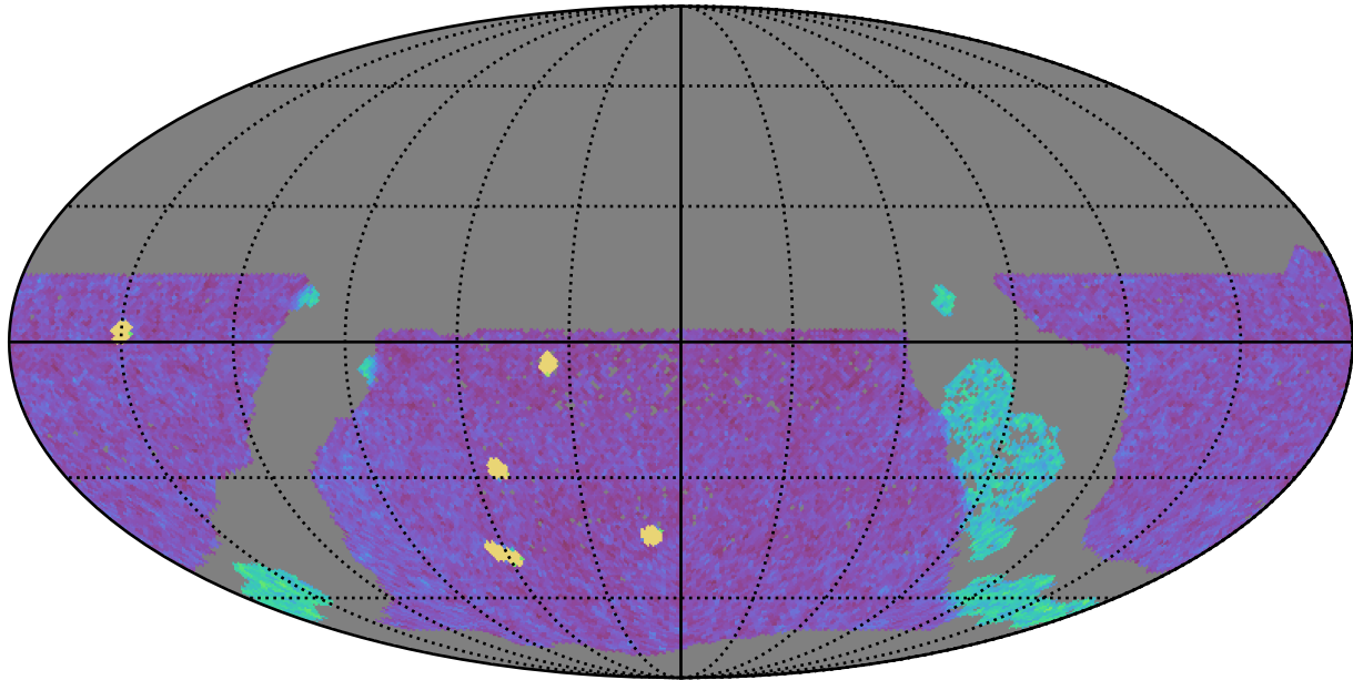
ddf_acor_sf10_lsf40_lsr20_v3.4_10yrs WFD g band: NVisits
