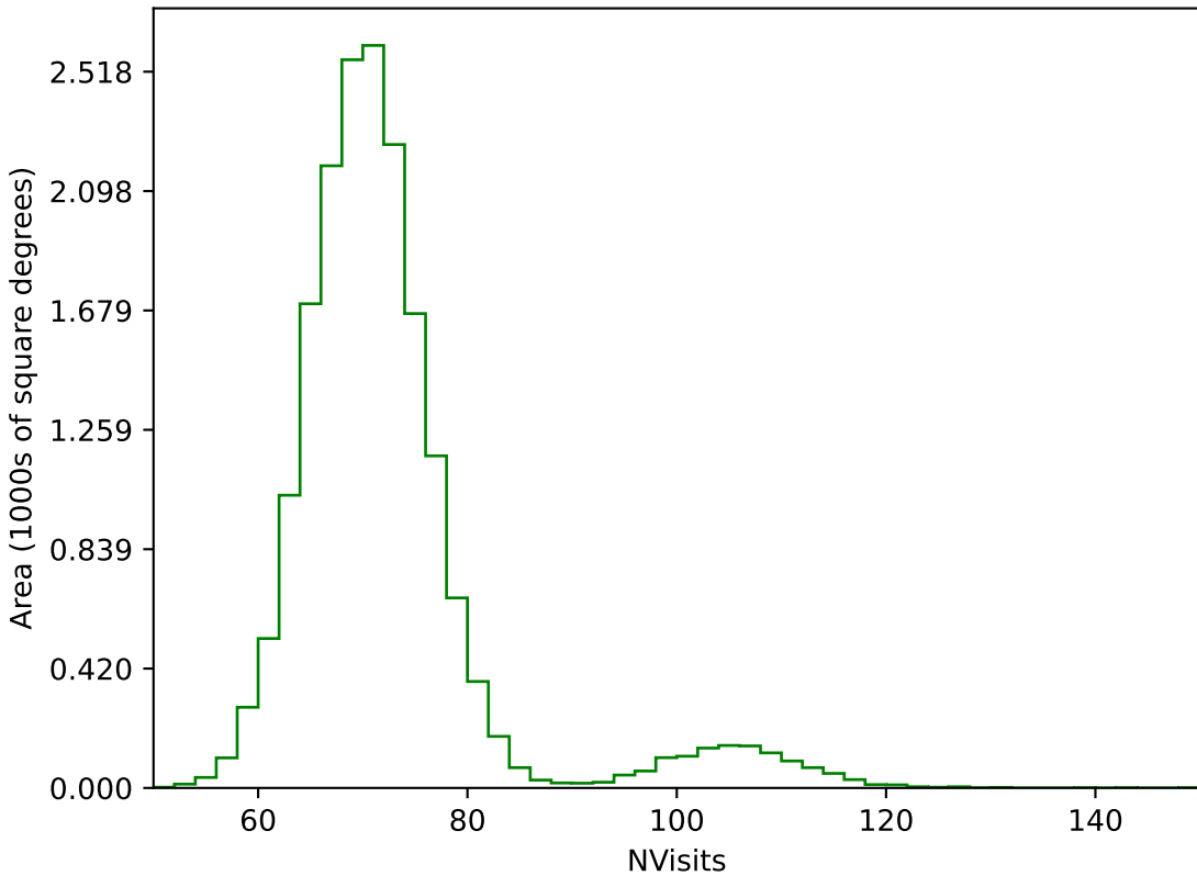
ddf_acor_sf10_lsf40_lsr20_v3.4_10yrs WFD g band: NVisits
