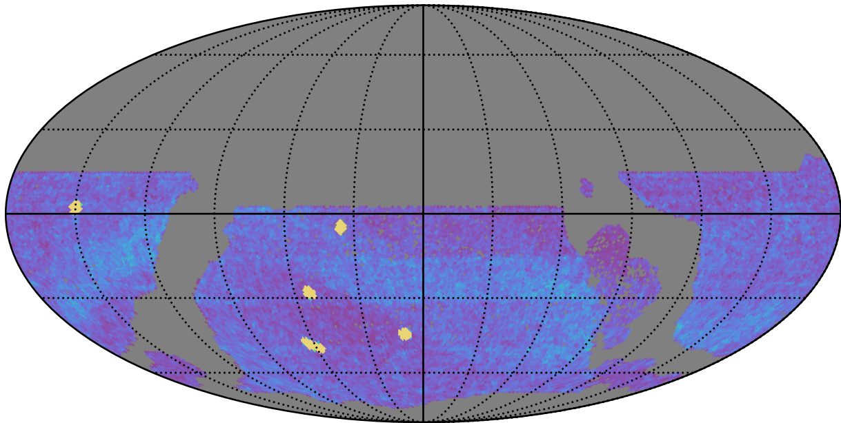
ddf_acor_sf10_lsf40_lsr20_v3.4_10yrs WFD all bands: NVisits
