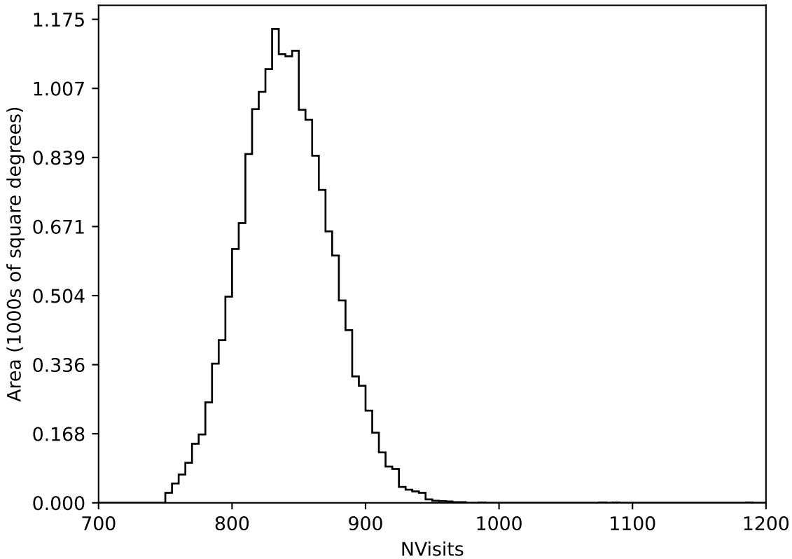
ddf_acor_sf10_lsf40_lsr20_v3.4_10yrs WFD all bands: NVisits
