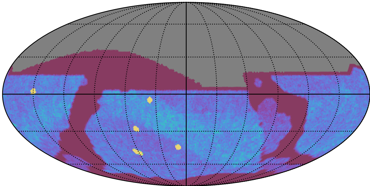
ddf_acor_sf10_lsf40_lsr20_v3.4_10yrs All sky z band: NVisits
