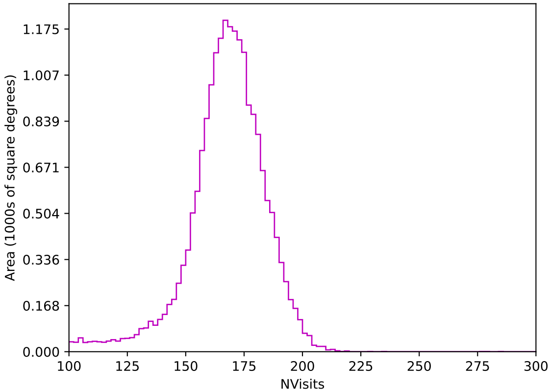
ddf_acor_sf10_ls40_lsr20_v3.4_10yrs All sky z band: NVisits
