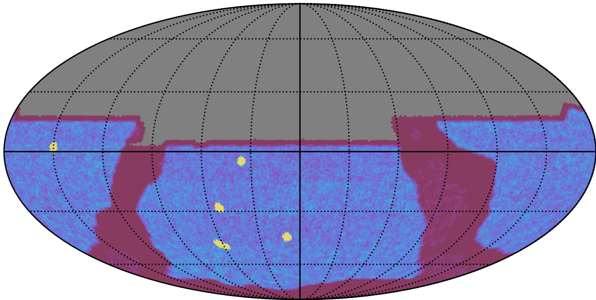
ddf_acor_sf10_lsf40_lsr20_v3.4_10yrs All sky y band: NVisits
