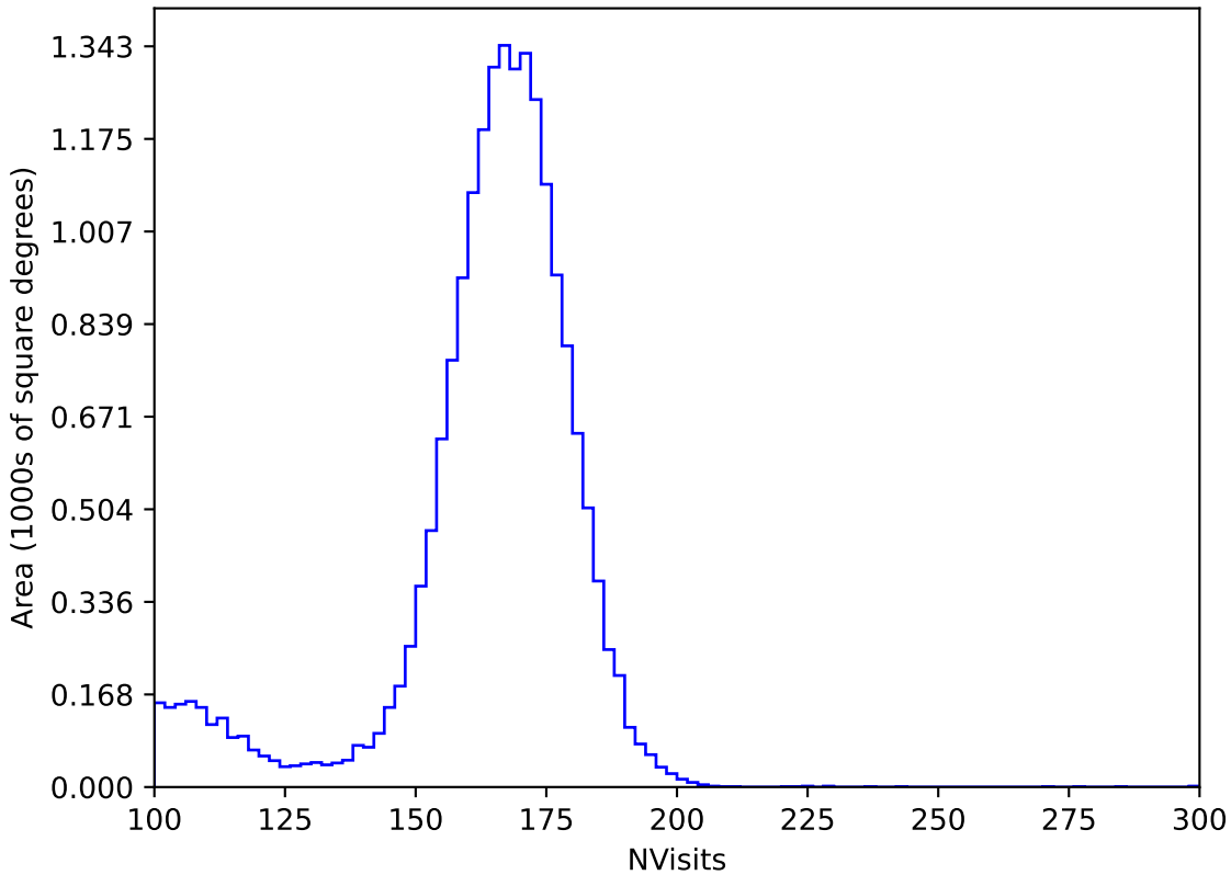
ddf_acor_sf10_ls40_lsr20_v3.4_10yrs All sky y band: NVisits
