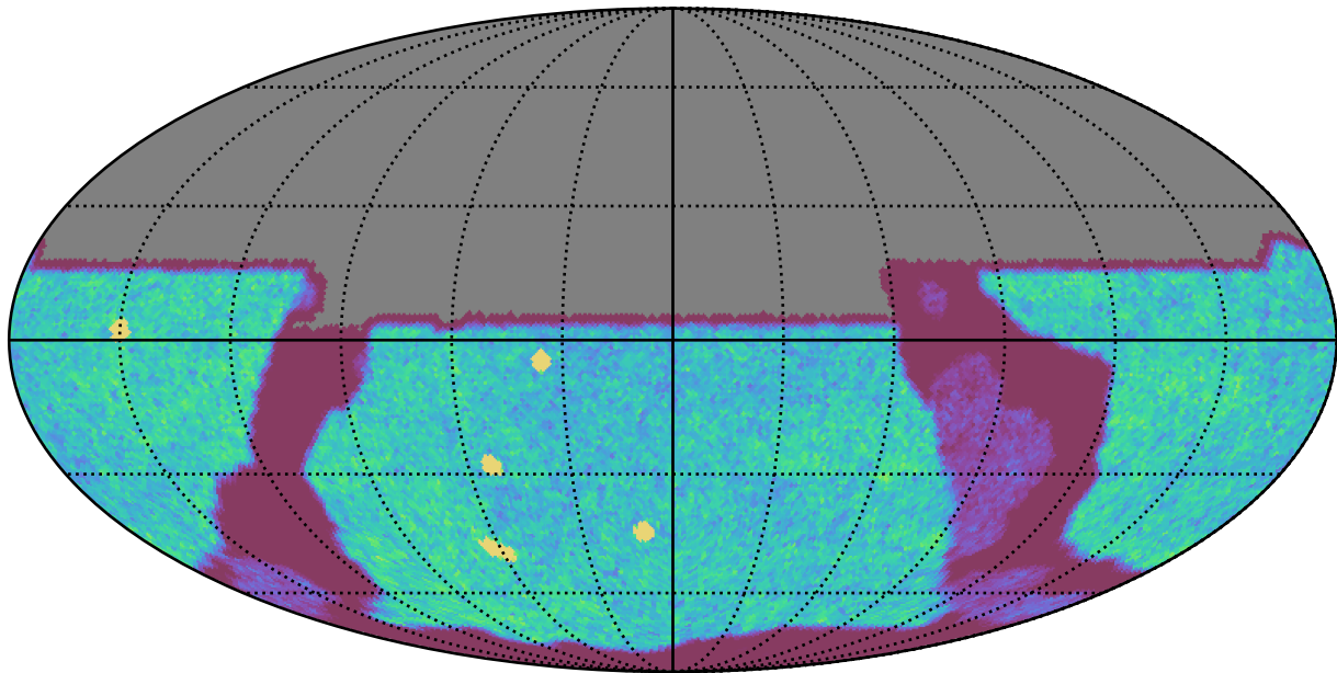
ddf_acor_sf10_lsf40_lsr20_v3.4_10yrs All sky u band: NVisits
