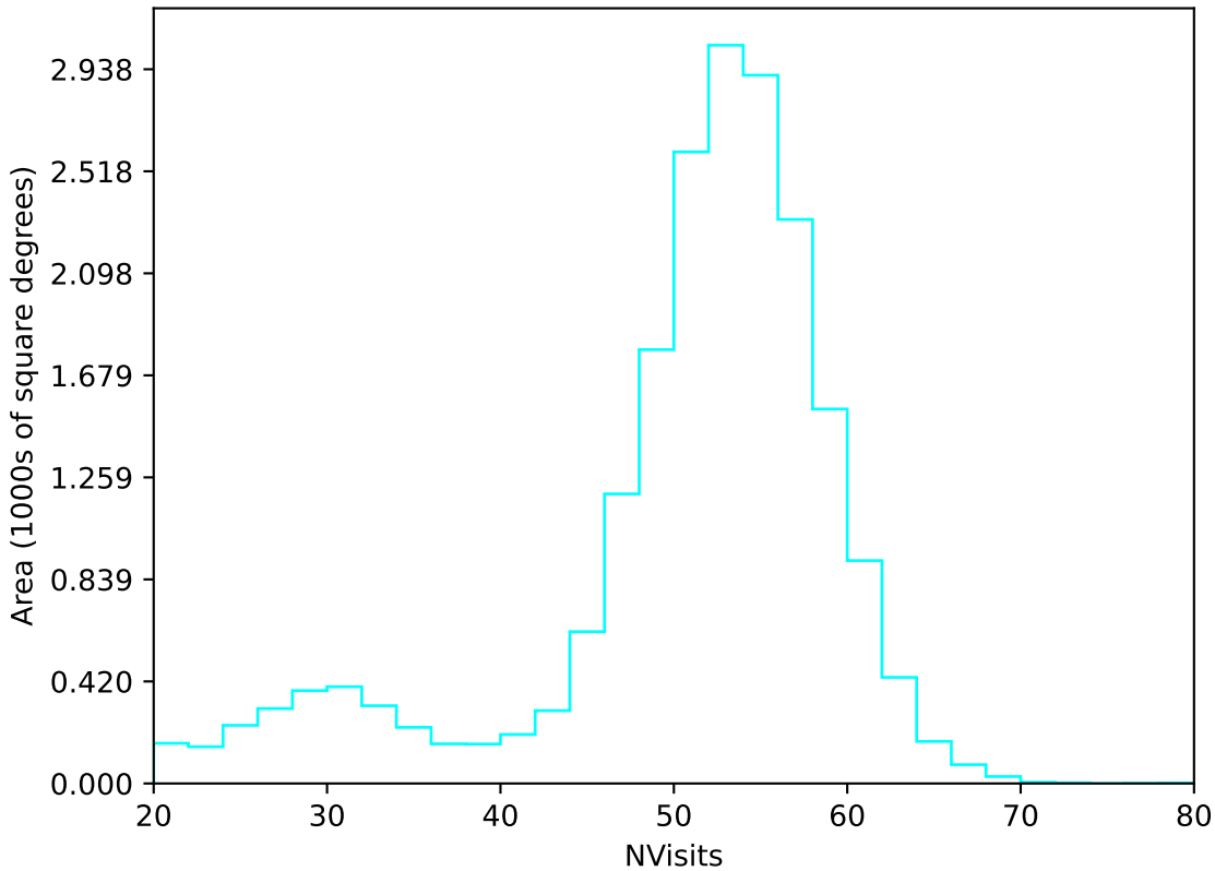
ddf_acor_sf10_lsf40_lsr20_v3.4_10yrs All sky u band: NVisits
