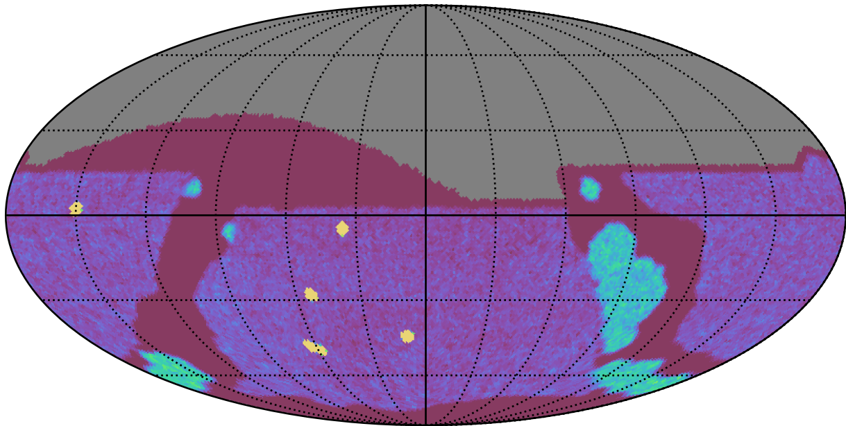
ddf_acor_sf10_lsf40_lsr20_v3.4_10yrs All sky g band: NVisits
