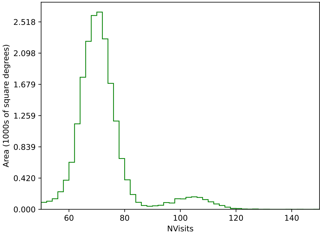
ddf_acor_sf10_lsf40_lsr20_v3.4_10yrs All sky g band: NVisits
