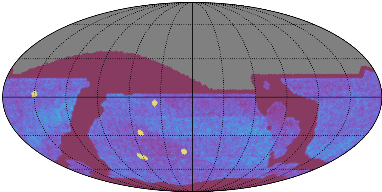
ddf_acor_sf10_lsf40_lsr20_v3.4_10yrs All sky all bands: NVisits
