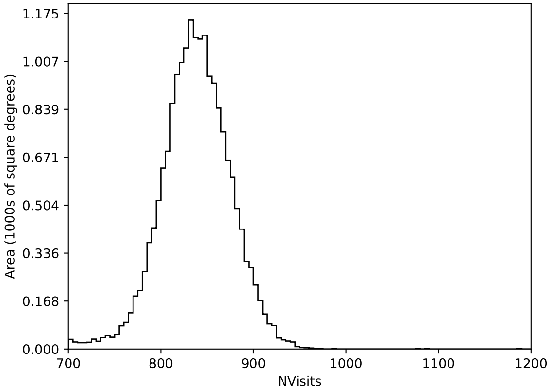
ddf_acor_sf10_lsf40_lsr20_v3.4_10yrs All sky all bands: NVisits
