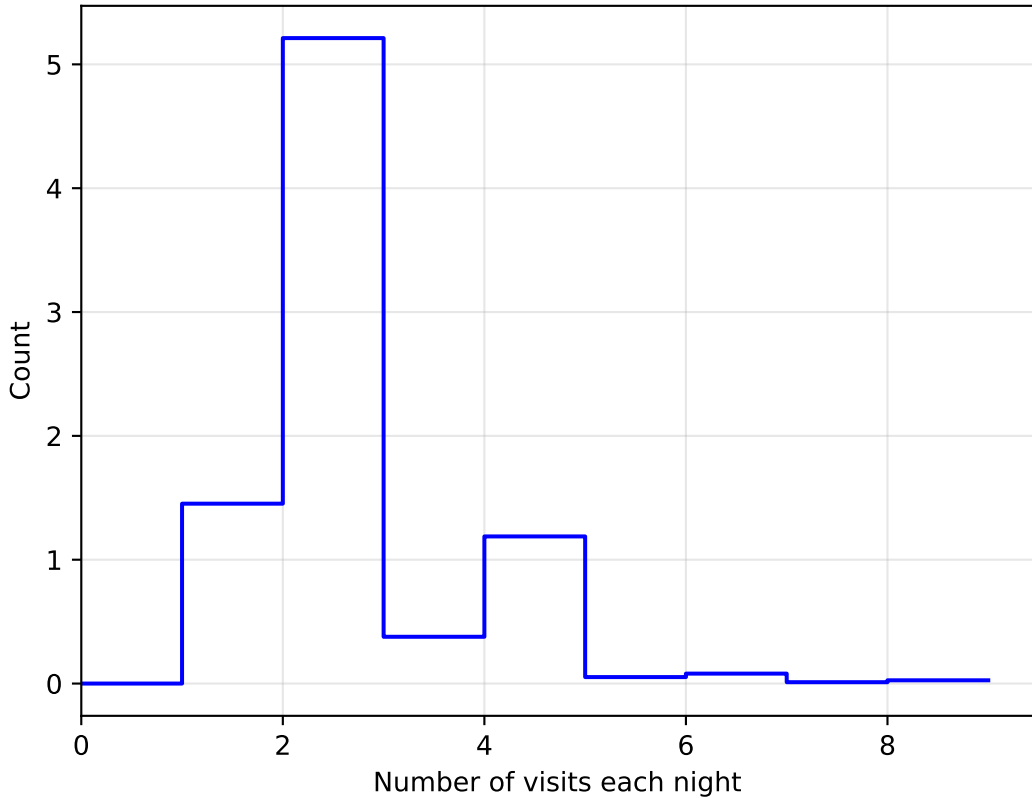
ddf_acor_sf10_lsf40_lsr20_v3.4_10yrs WFD: NVisitsPerNight 1e6
