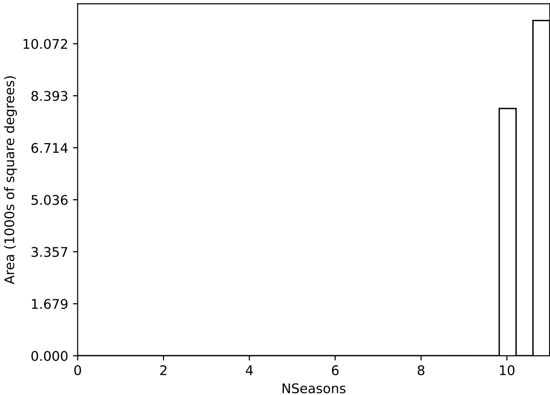
ddf_acor_sf10_lsf40_lsr20_v3.4_10yrs WFD all bands: NSeasons
