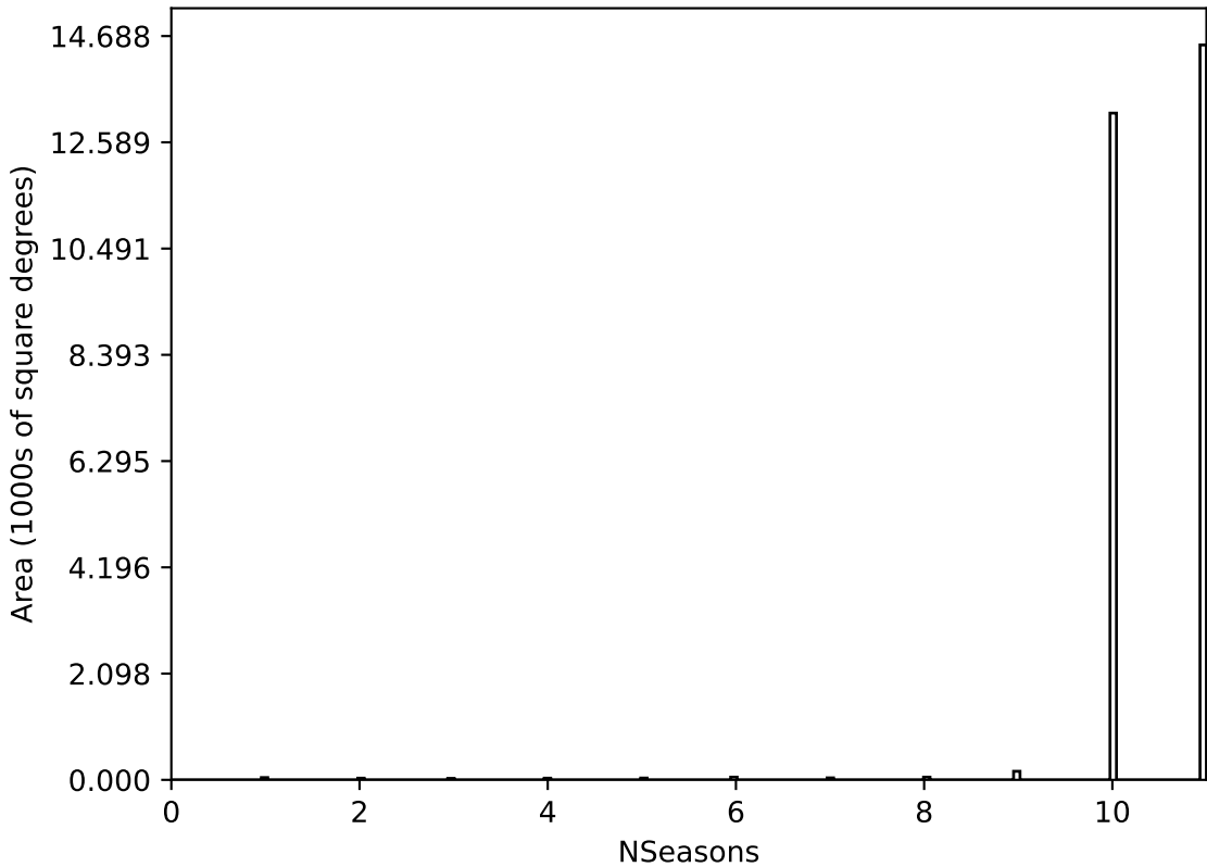
ddf_acor_sf10_lsf40_lsr20_v3.4_10yrs All sky all bands: NSeasons
