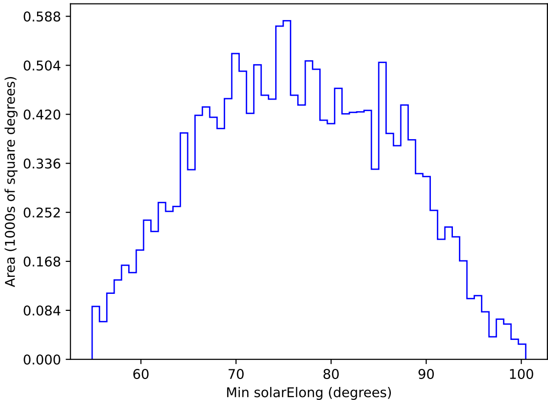
ddf_acor_sf10_lsf40_lsr20_v3.4_10yrs WFD u band: Min solarElong
