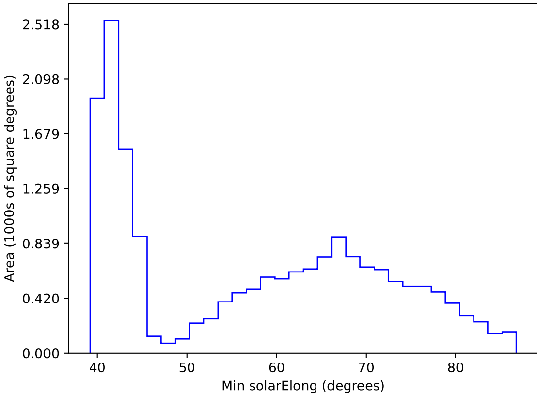
ddf_acor_sf10_lsf40_lsr20_v3.4_10yrs WFD r band: Min solarElong
