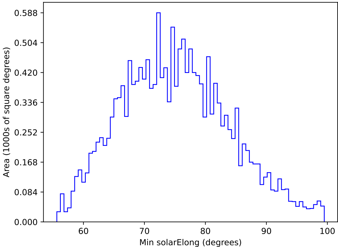
ddf_acor_sf10_lsf40_lsr20_v3.4_10yrs WFD g band: Min solarElong
