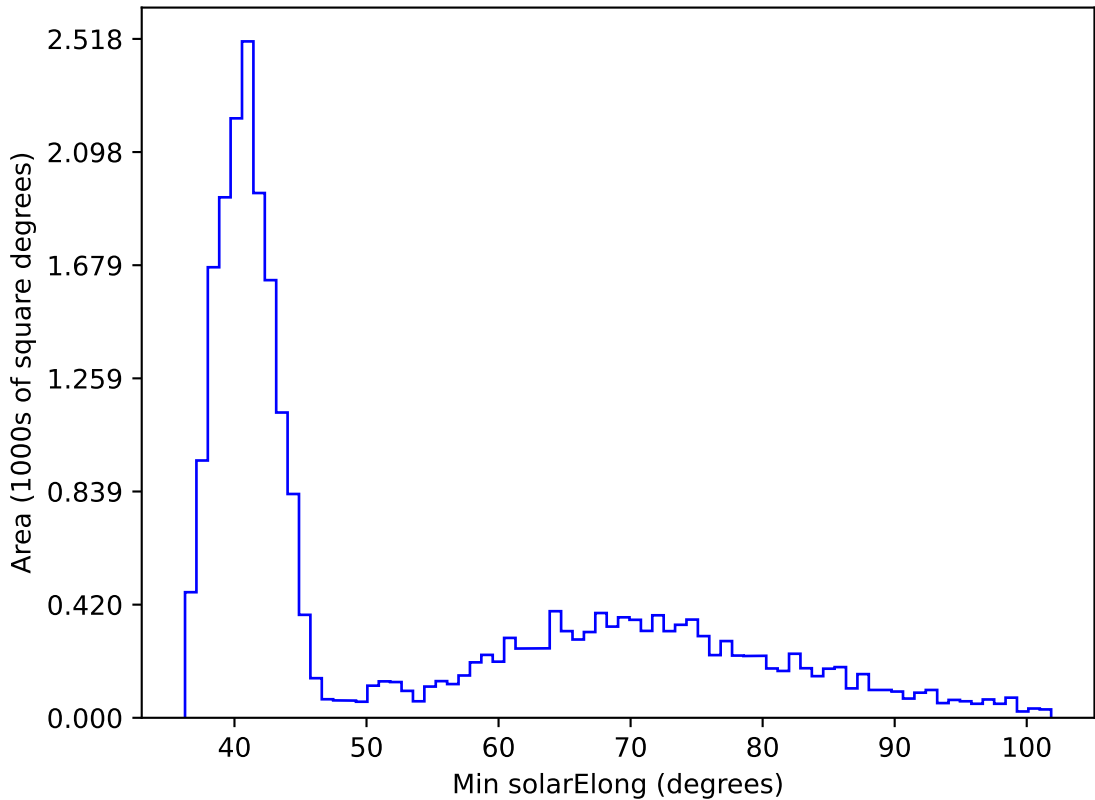
ddf_acor_sf10_lsf40_lsr20_v3.4_10yrs All sky z band: Min solarElong
