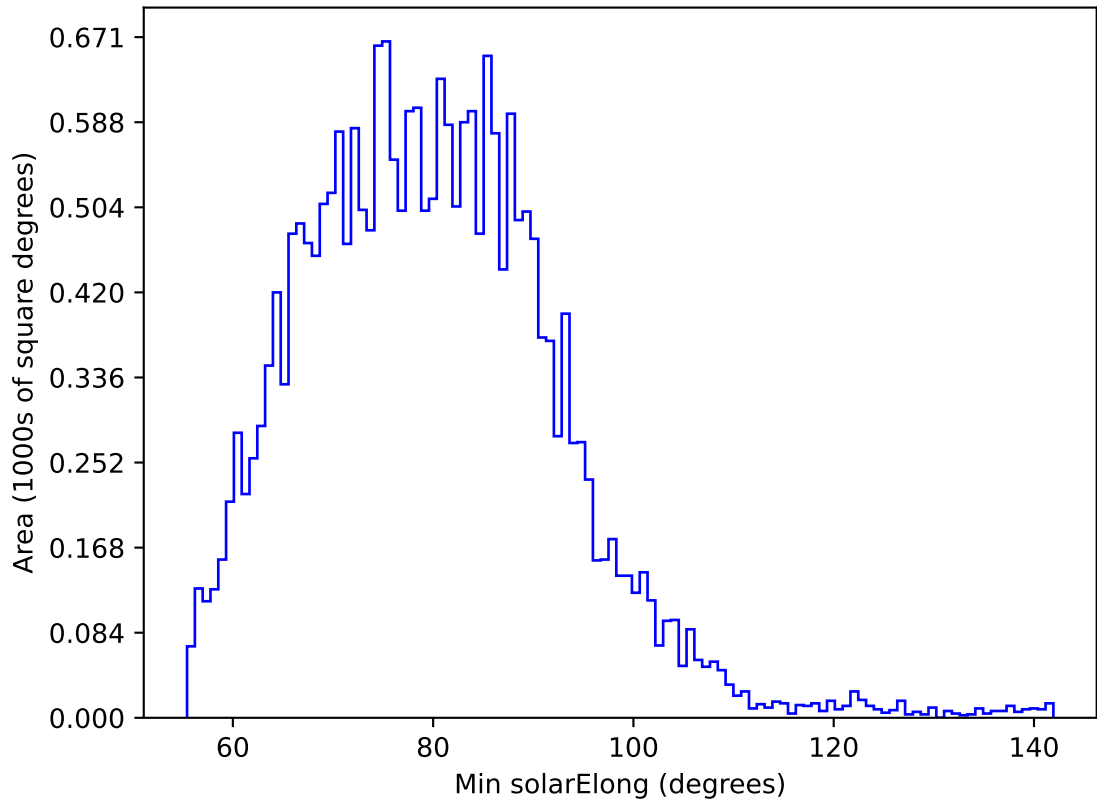
ddf_acor_sf10_lsf40_lsr20_v3.4_10yrs All sky u band: Min solarElong
