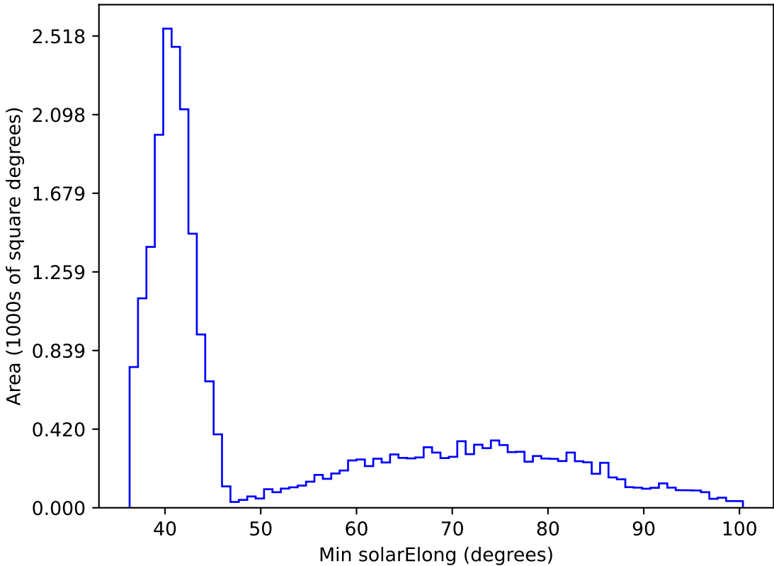
ddf_acor_sf10_lsf40_lsr20_v3.4_10yrs All sky i band: Min solarElong
