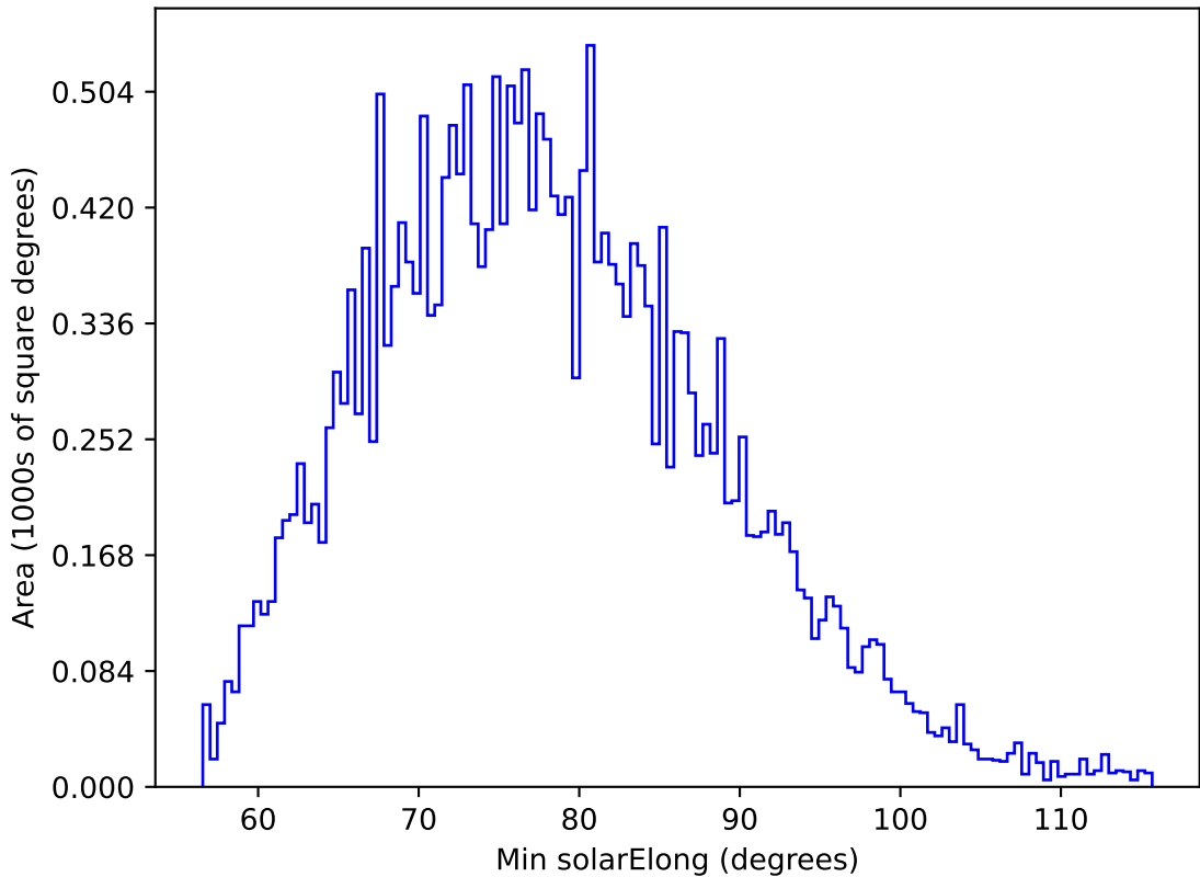
ddf_acor_sf10_lsf40_lsr20_v3.4_10yrs All sky g band: Min solarElong
