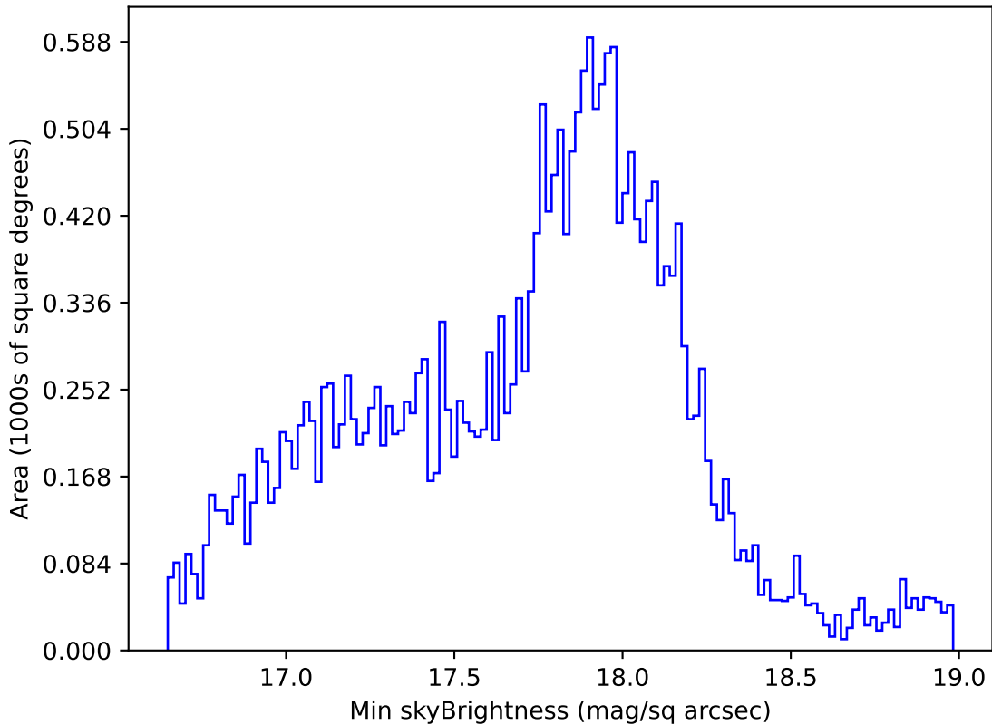
ddf_acor_sf10_lsf40_lsr20_v3.4_10yrs Yr 1 all bands: Min skyBrightness
