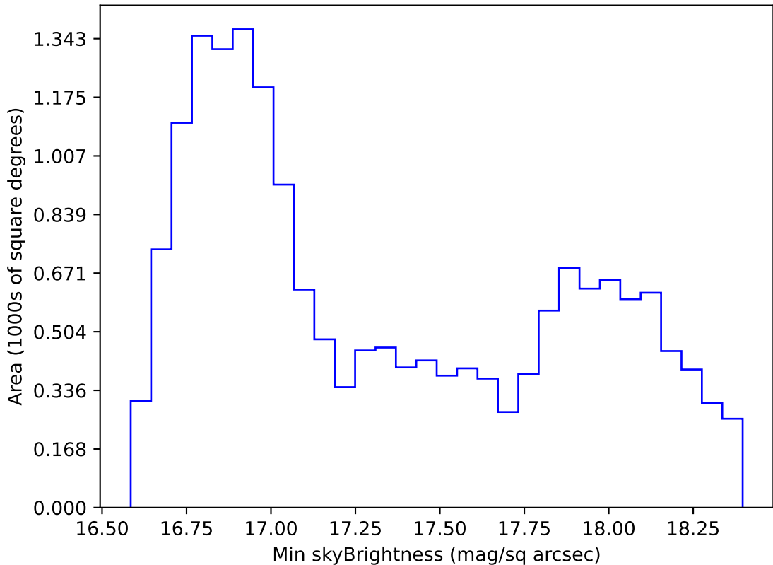
ddf_acor_sf10_lsf40_lsr20_v3.4_10yrs WFD z band: Min skyBrightness
