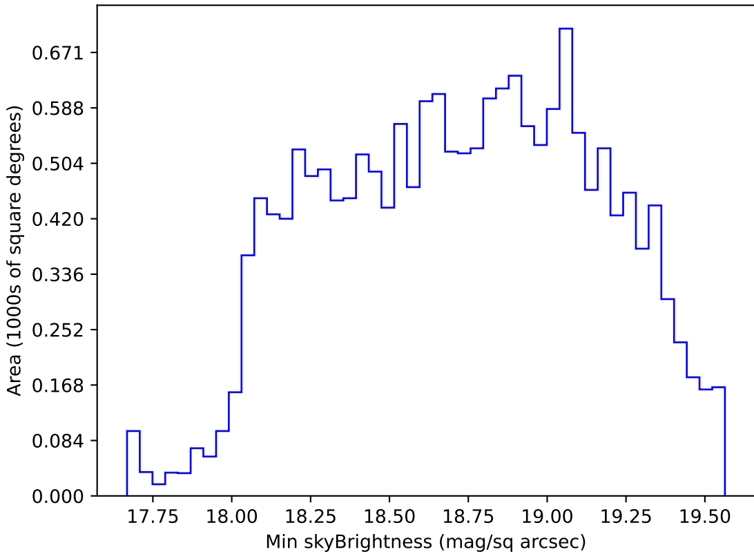
ddf_acor_sf10_lsf40_lsr20_v3.4_10yrs WFD r band: Min skyBrightness
