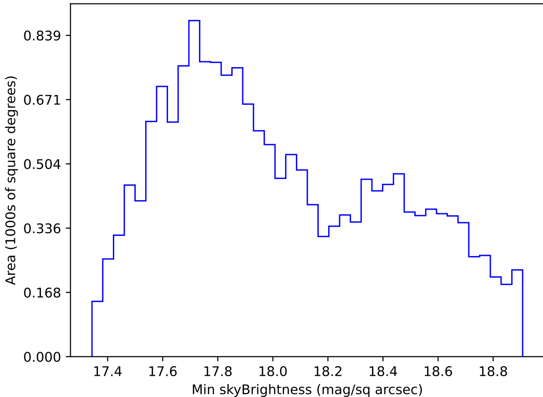
ddf_acor_sf10_lsf40_lsr20_v3.4_10yrs WFD i band: Min skyBrightness
